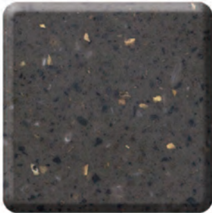
Meteorite
